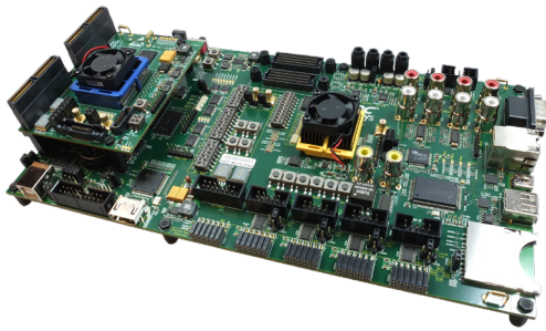
Figure 5: ARC AXS103 Software Development Platform
