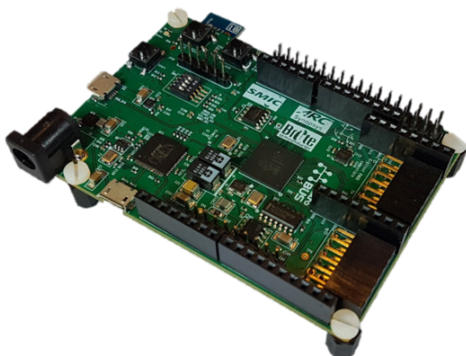
Figure 2: ARC IoT Development Kit
